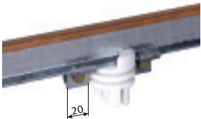
Illustration shows an insulator with 2 locating clamps (fix point)
