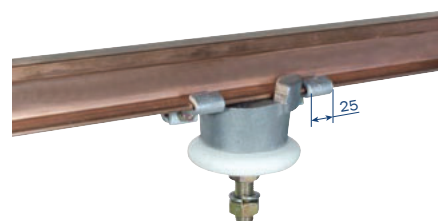
Illustration shows an insulator with 2 locating clamps (fix point)
