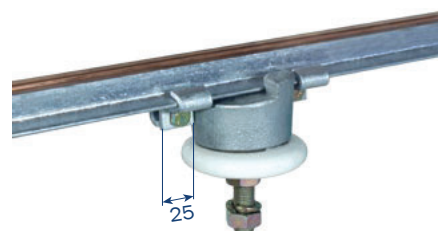
Illustration shows an insulator with 2 locating clamps (fix point)
