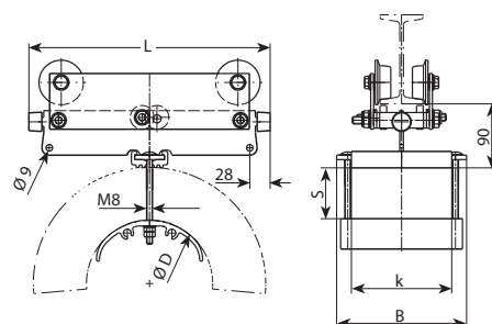
Collecting clamp for round cables Extension rubber profile can be ordered per meter (Order-no.: 348 845)
