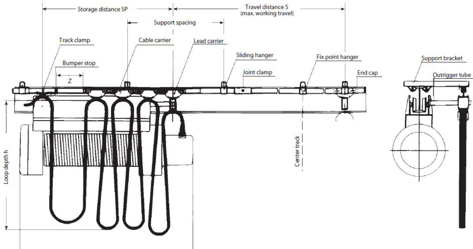
C-Track
